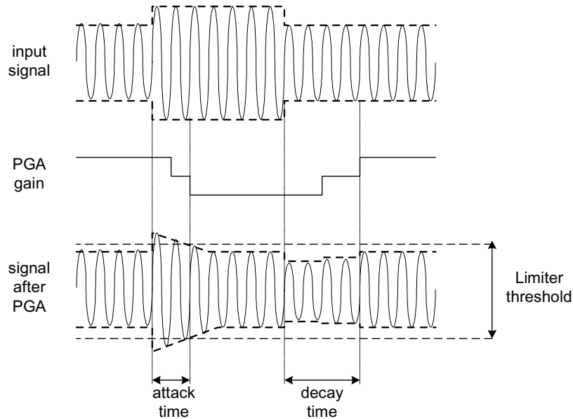
Figure 22 Limiter Operation
