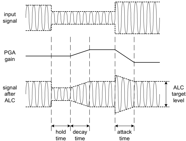
Figure 23 ALC Operation
