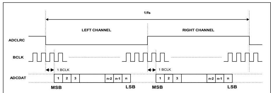
Figure 14 I^2S Mode
