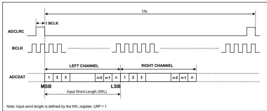
Figure 16 DSP Mode
