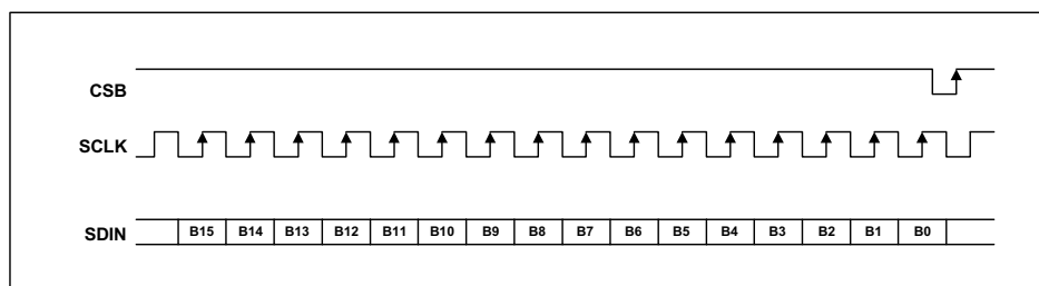
Figure 19 3-Wire Serial Interface
